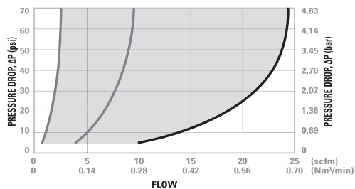
20CB Series Air Flow
