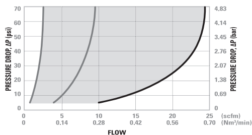
20AC Series Air Flow
