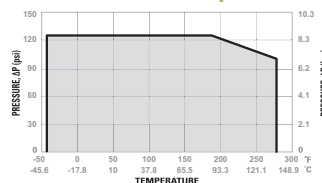
60PS Series Temperature
