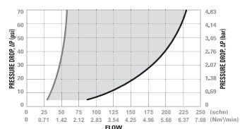
60PS Series Air Flow
