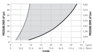
60PS Series Water Flow
