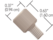
LT-110 10-32 PEEK Nut for 1/32" and 1/16" OD tubing
