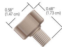
LT-210 1/4-28 PEEK Double-Winged Nut for 1/8" OD tubing
