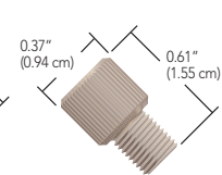
LT-215 1/4-28 PEEK Nut for 1/8" OD tubing
