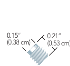
F-354 10-32 Stainless Steel FlushNut for 1/32" and 1/16" OD tubing
