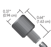
F-195 10-32 Short PEEK Nut, with F-192 Ferrule
