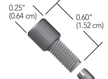
F-198 10-32 Short PEEK Headless Nut, with F-192 Ferrule
