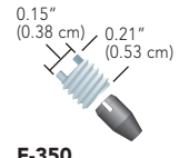
F-350 10-32 Stainless Steel FlushNut, with F-192 Ferrule
